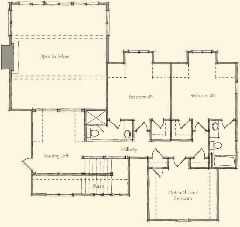
Optional Upper Level INSPIRATION HOME 1,468 Heated Sq. Ft.
