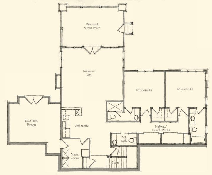
Lake Level INSPIRATION HOME 1,468 Heated Sq. Ft.
